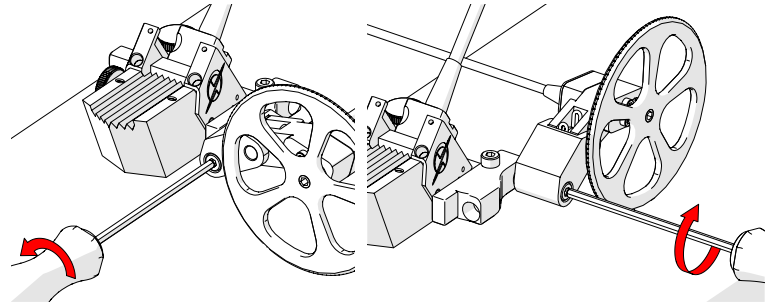
Fig. 7 - Unscrew pivot knob and remove encoder
