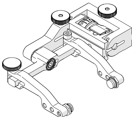
Fig. 4 - Slip joint probe holder
