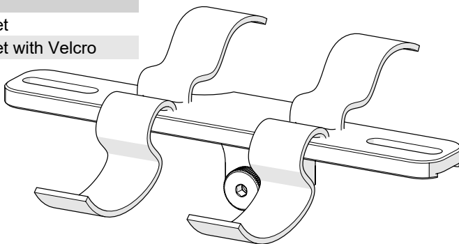
Fig. 88 - Preamp bracket
