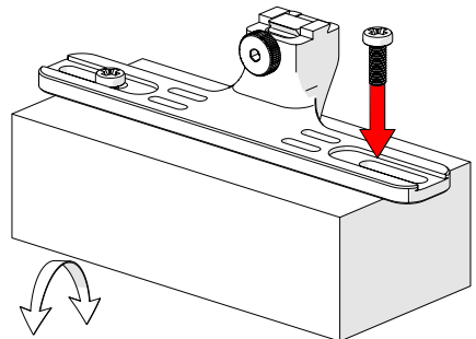
Fig. 78 - Attach preamp with screws
