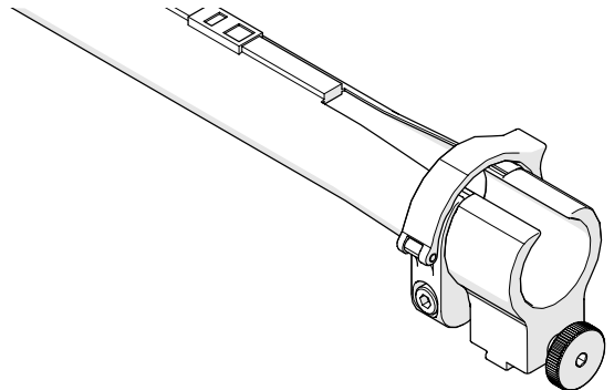
Fig. 16 - Cable management
