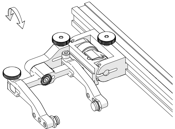
Fig. 64 - Reversed probe holder
