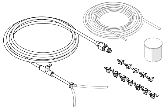
Fig. 7 - Irrigation kit
