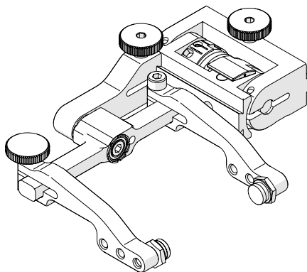
Fig. 10 - Slip joint probe holder
