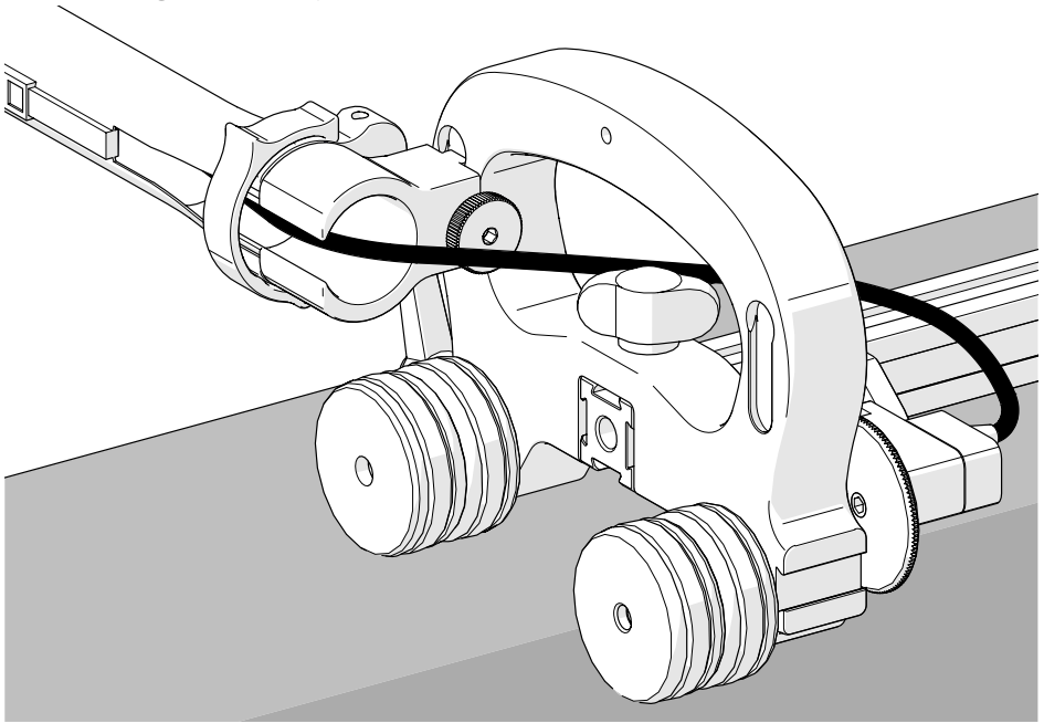
Fig. 67 - Cable management
