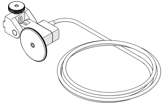
Fig. 6 - Spring-loaded encoder
